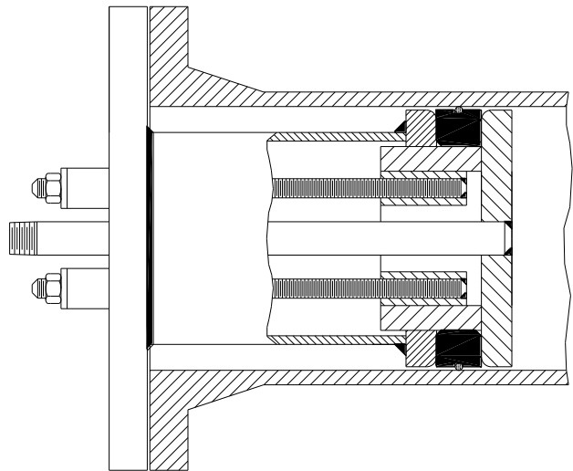
Figure 4. Flange Test Plugs Installed as Isolation Plug.
