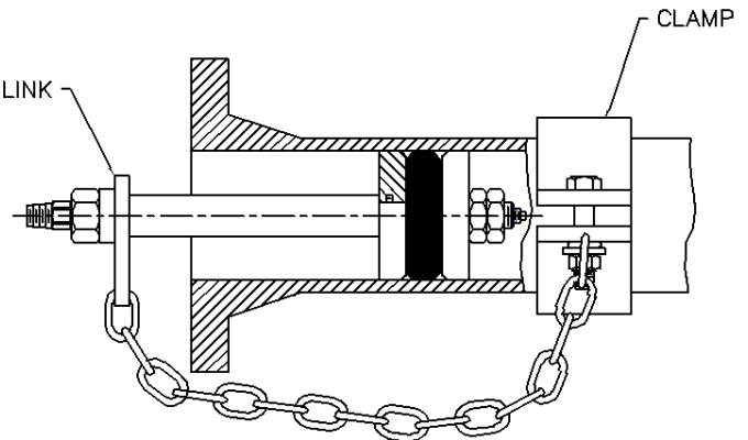
Figure 2. Flange Test Plugs Installed as Isolation Plug, After Flange Has Been Removed.
