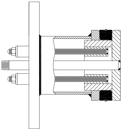
Figure 3. Flange Test Plug With Flange Installed.
